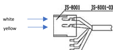
Picture 4 – 0.17kW EC drives control cable pinout
