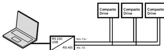
Picture 8 - "daisy chain" connection
