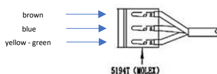
Picture 3 – 0.17kW EC drives power cable pinout
