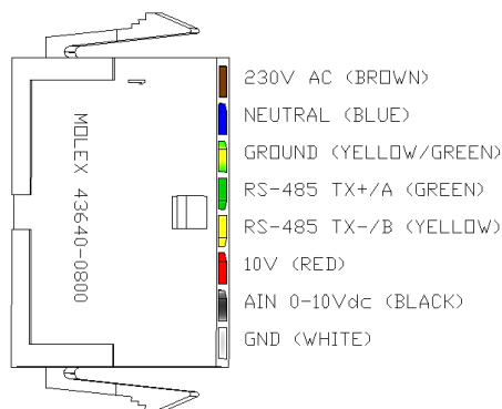
Picture 5 - 0.37 / 0.75kW EC drives power - control cable pinout
